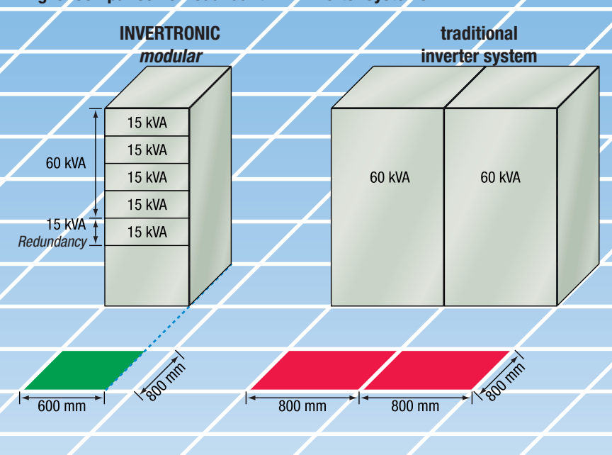
Fig. 6: Comparison of redundant n+1 inverter systems
