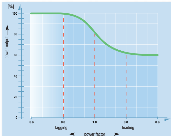
Fig. 8: Available inverter apparent output power depending on power factor
